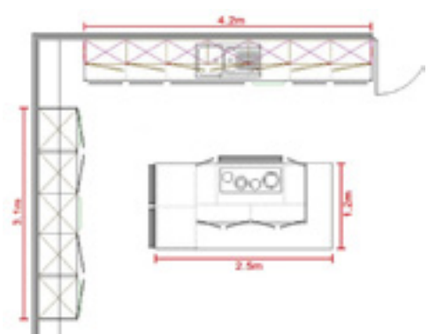
True handleless mix, L-Shape kitchen with rectangular island, finished height 2300mm.
