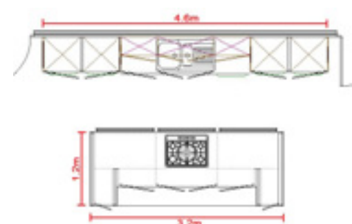
True handleless In-Line wall section with island, finished height 2300mm + bulkhead surround.
