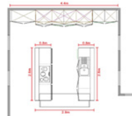
Contemporary C: In-Line wall to wall section with double linked island, finished height: 2300mm + 360 top cabinets.
