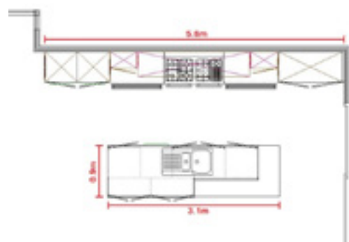
In-Line wall section with rectangular island, finished height 2120mm + 360mm top glazed cabinets. (2480mm total)
