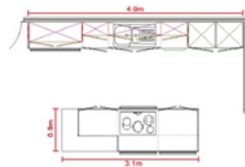
True handleless, In-Line wall section with rectangular island, finished height 2300mm.
