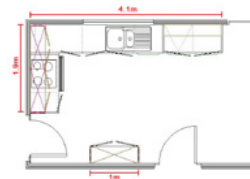
L-Shape kitchen + separate slim stand-alone larder, finished height: 2300mm.
