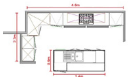
L-Shape kitchen, with Corner larder & Midi height ovens, finished height: 2300mm.
